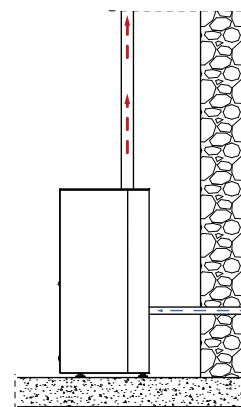
Installation Typ "b" *
