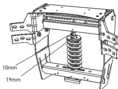
CHARNIÈRE ALTERNATIVE
